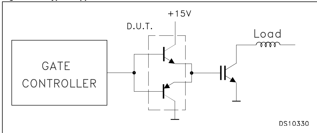
Figure 11. Typical application
